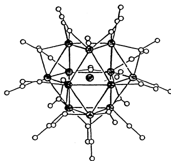
Fig. 2. The molecular structure of [\text{H}_3\text{Rh}_{13}(\text{CO})_{24}]^{2-} .
