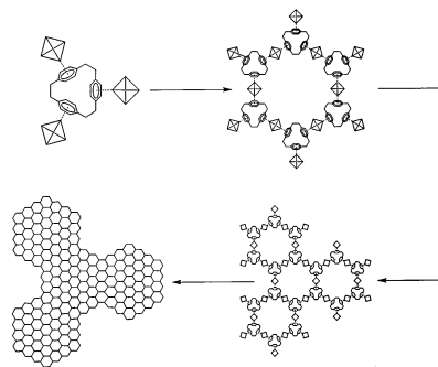
Fig. 8. Linked cobalt clusters.
